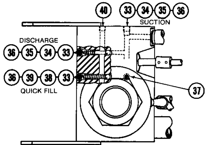
BASE ASSY. - TOP VIEW
