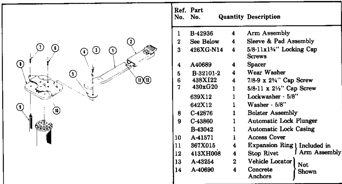
FIGURE 4-1. FS-10 SUPERSTRUCTURE ASSEMBLY
