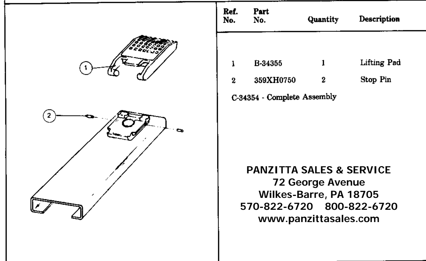
FIGURE 4-2. PAD AND SLEEVE ASSEMBLY (4 POSITION)
