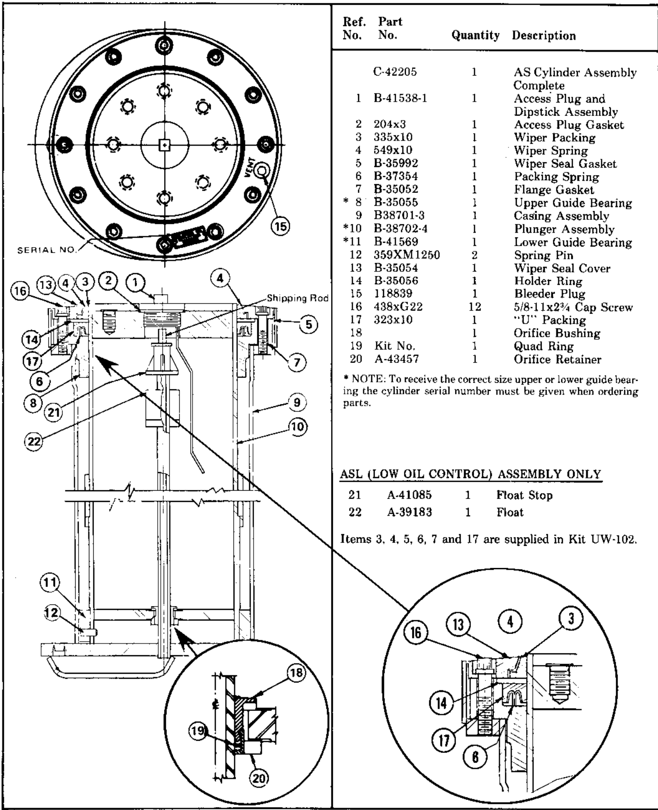
FIGURE 4-4. AS CYLINDER ASSEMBLY Semi-Hydraulic Type "WB" Cylinder (67 1/2" Stroke)
